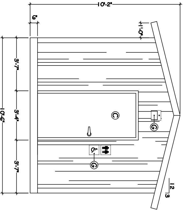
FRONT ELEVATION
