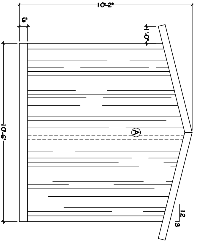
REAR ELEVATION
