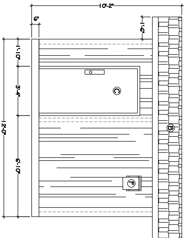
LEFT ELEVATION
