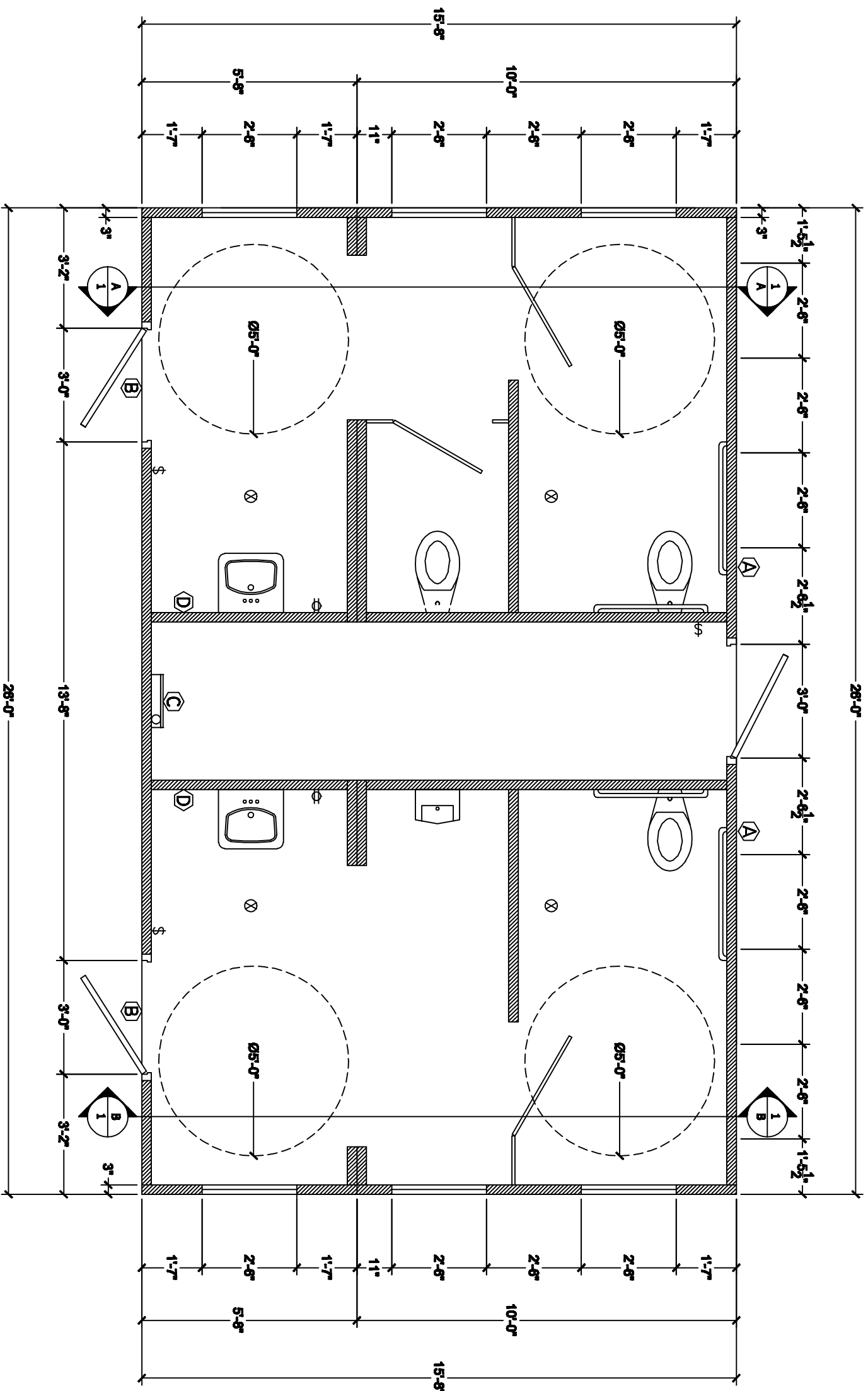
PLAN VIEW
