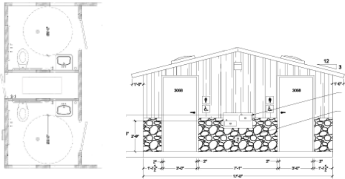
WILLOUGHBY Male/female with chase [ADA]
