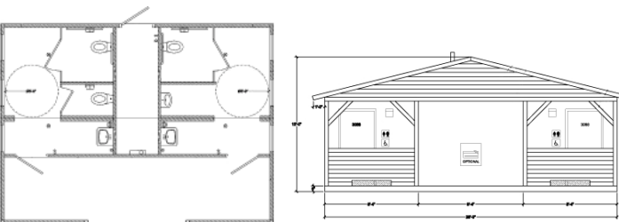
MOUNTAINEER Male/female with chase [ADA]
