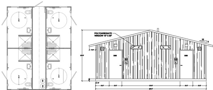
POTOMAC Male/female with shower [ADA]
