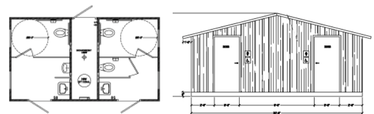
ALLEGHENY Male/female with chase [ADA]
